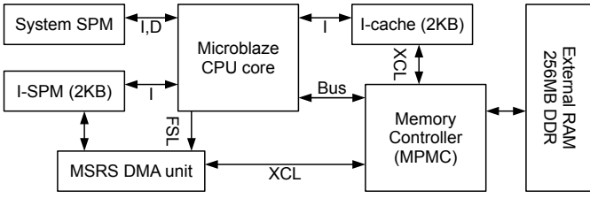
Fig. 2. Microblaze+SPM hardware implemented within an FPGA.
